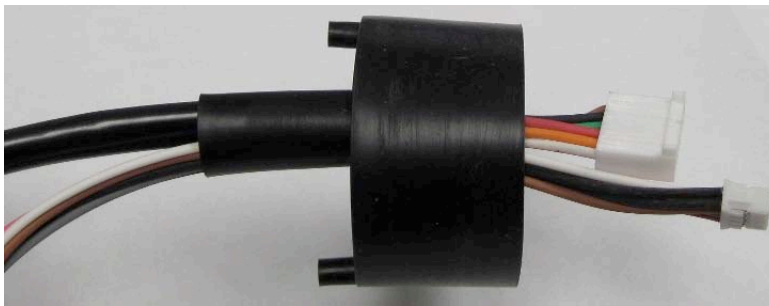
Figure 1. Insert Harnesses
